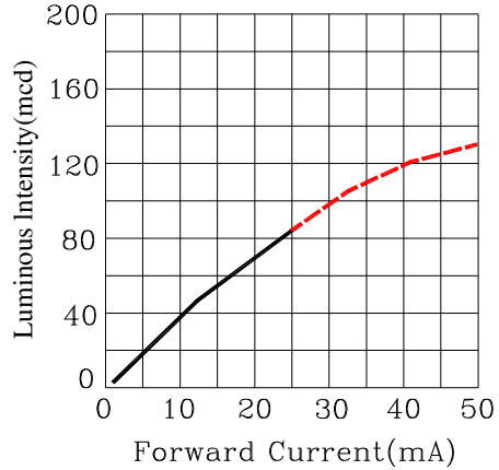
Fig.3 Luminous Intensity vs. Forward Current
