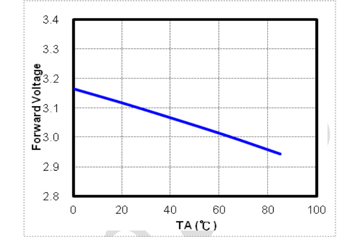
6. Forward Voltage vs. Ambient Temperature ( I_F=120\text{mA} )
