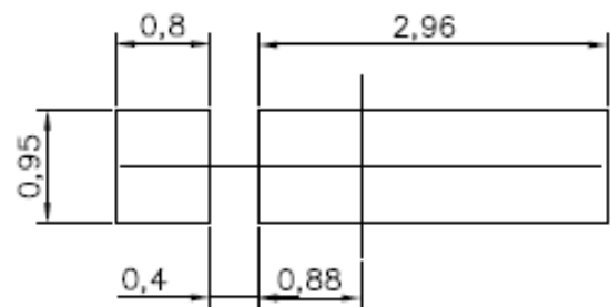
Soldering patterns
