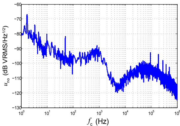
Figure 3: Typical noise voltage spectral density referred to primary u_{no} with R_M = 100 \text{ } \Omega
