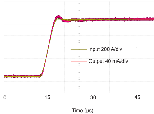
Figure 2: Typical step response (0 to 1 kA, 200 A/μs)
