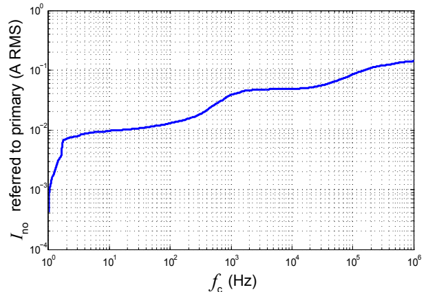
Figure 4: Typical RMS noise current referred to primary I_{no} with R_M = 100 \text{ } \Omega
