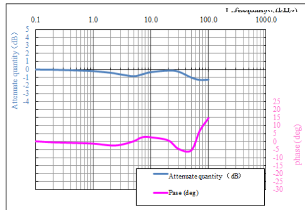
Figure 2: Frequency response curve
