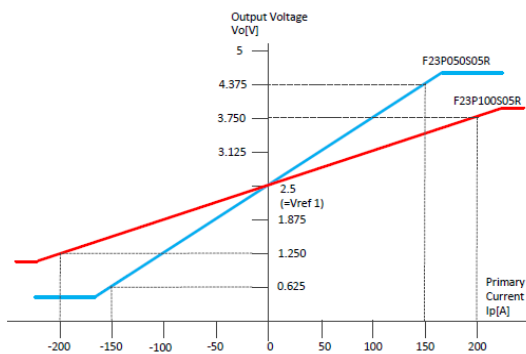
Figure 1: Linearity curve (Internal reference voltage)
