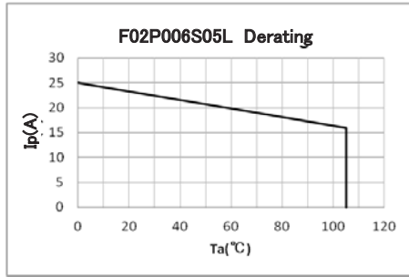
Figure 3: Ip vs Ta for F02P006S05L
