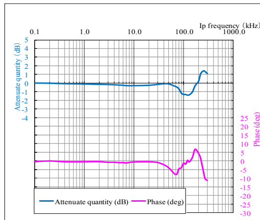
Figure 2: Frequency response curve ex) F02P025S05L Measurement condition T A =+25°C, R L =1kΩ, I p =3A, V CC =+5V
