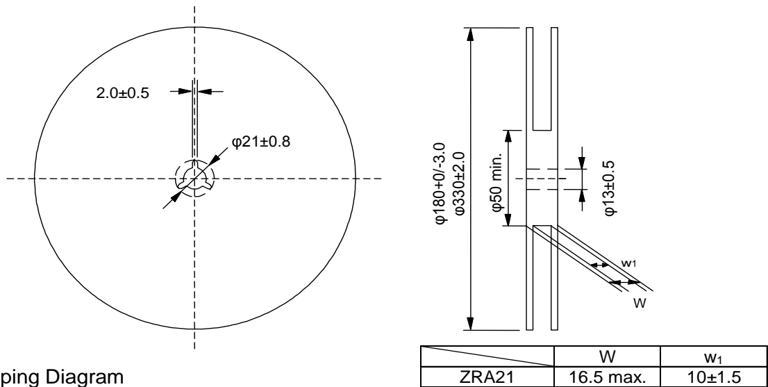
Fig.2 Dimensions of Reel
